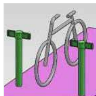
13842 X-Last Bollard 100 + 2 Arms Bike Slow Point Using X-Last Recovering, Impact Tested Bollards
