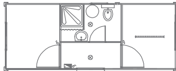
▲ 1157 Office container, 6,0 x 2,4 m, two spaces and lobby with toilet, wash basin and shower, 4 doors, 3 windows, Insulated, PVC floor, cables, fuses, 5 socket, 3 ceiling lights and hot water unit
