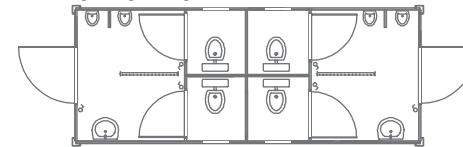
▲ 1194 sanitary container 6,0 x 2,4 m Insulated, two wash basins, 4 urinals, 4 Toilet cubicles, ceiling lights, PVC floor
