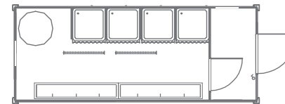
▲ 1195 sanitary container dimensions 6,0 x 2,4 m, Insulated, two doors, 4 shower cabins, hot water unit, 2 washing basins, ceiling lights, PVC floor
