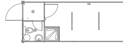
▲ 1106 Office container 6,0 x 2,4 m with lobby and equipped toilet and shower, two doors, three windows, Insulated, cables, fuses, two ceiling lights, two sockets, 1 basin, PVC floor
