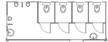
▲ 1192 sanitary container 6,0 x 2,4 m Insulated, 2 wash basins, 3 urinals, 4 Toilet cubicles, PVC floor
