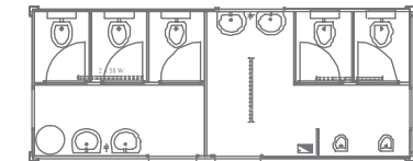
▲ 1107 sanitary container 6,0 x 2,4 m itwo spaces: 5 Toilet cubicles, 4 wash basins, 2 urinals, one Hot water unit, Tiled floor, Insulated,
