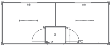
▲ 1141 Office container, 6,0 x 2,4 m, itwo spaces and lobby, 3 doors, 2 windows, Insulated, PVC floor, cables, fuses, 5 sockets, 3 ceiling lights
