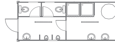
▲ 1191 sanitary container 6,0 x 2,4 Insulated, 2 toilet cabins, 3 wash basins, 2 urinals, 2 shower cubicles PVC floor
