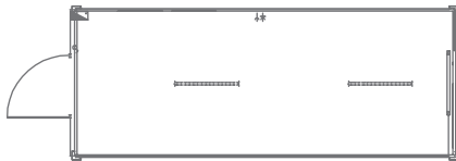
▲ 1148 Office container 6,0 x 2,4 m Insulated, door, cables, fuses, sockets, 2 ceiling lights, PVC floor
